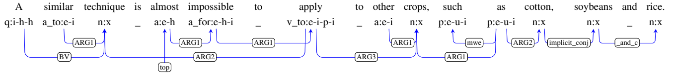
Representation 1: Minimal Recursion Semantics-derived dependencies (DM), from DeepBank HPSG annotation.
