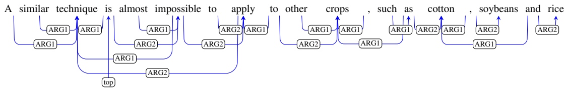
Representation 2: Predicate-argument structures (PAS), from Enju HPSG annotation.
